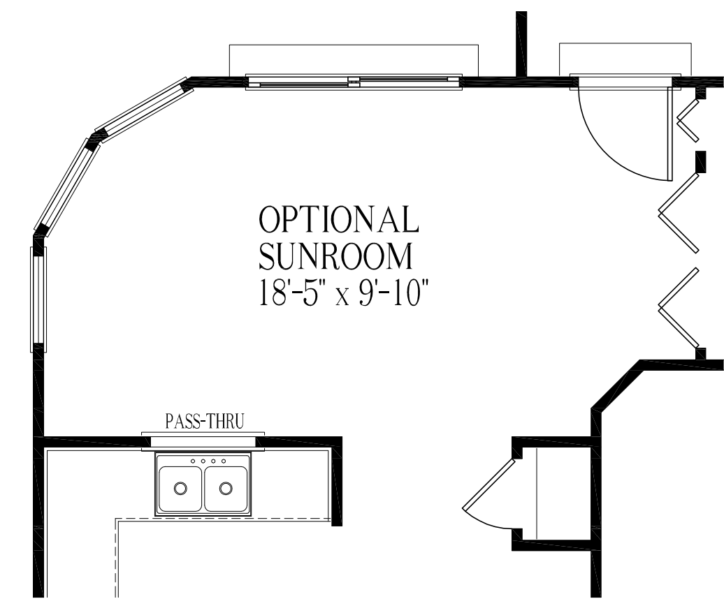
First Floor Plan - Optional Sunroom
