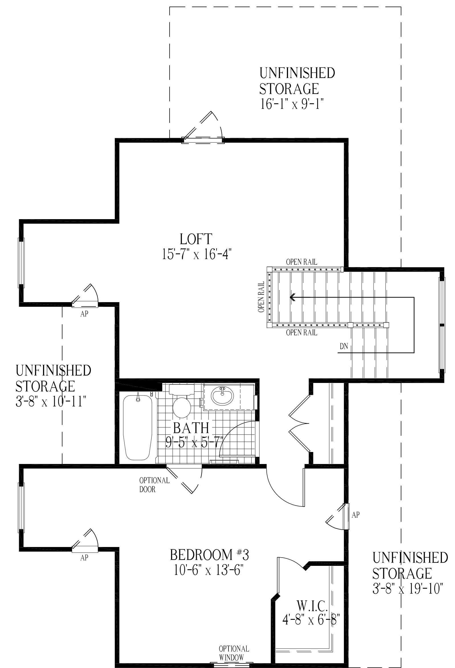
Second Floor Plan - Option No. 2 737 GSF
