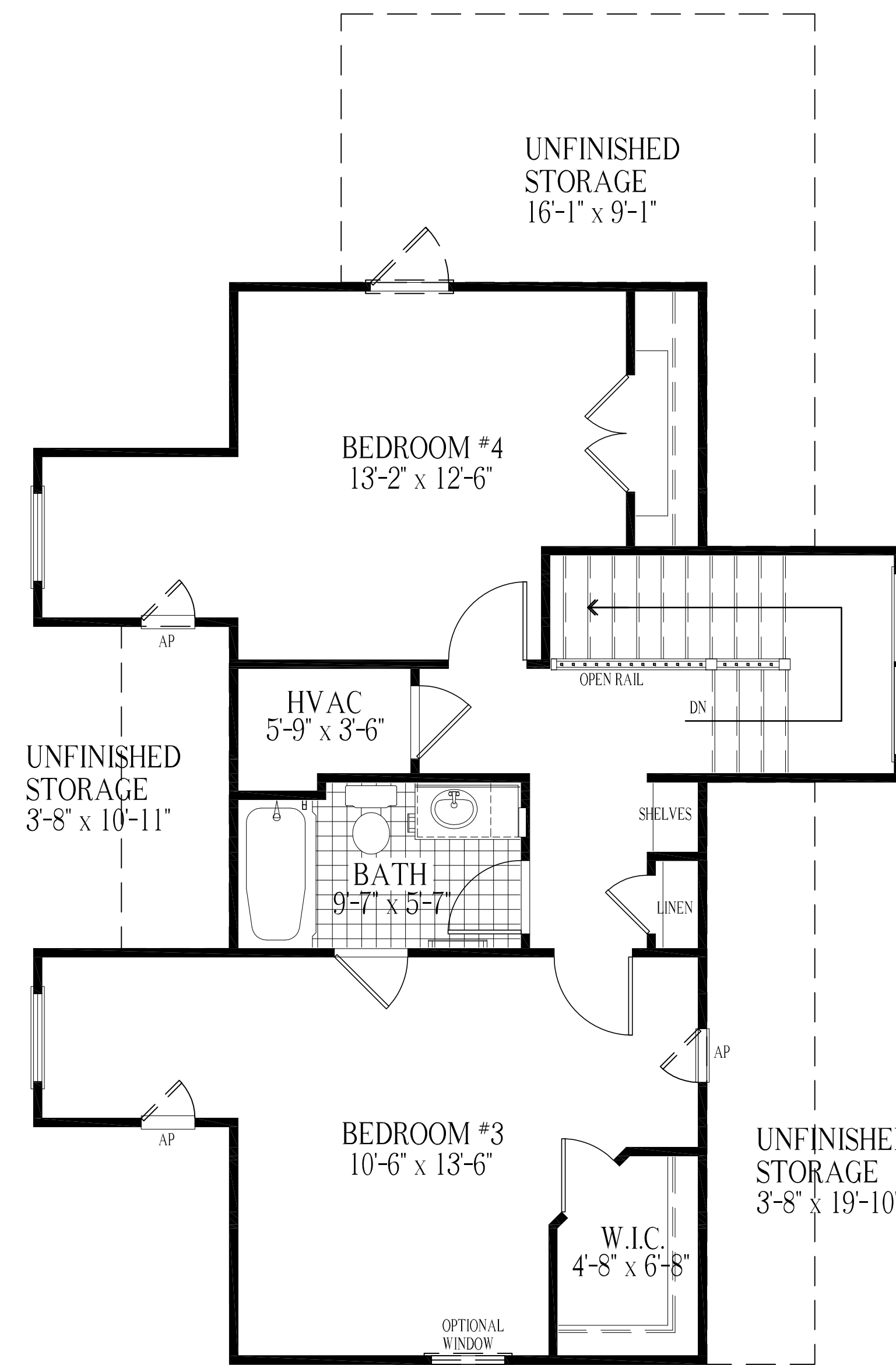
Second Floor Elevation 'A' 737 GSF
