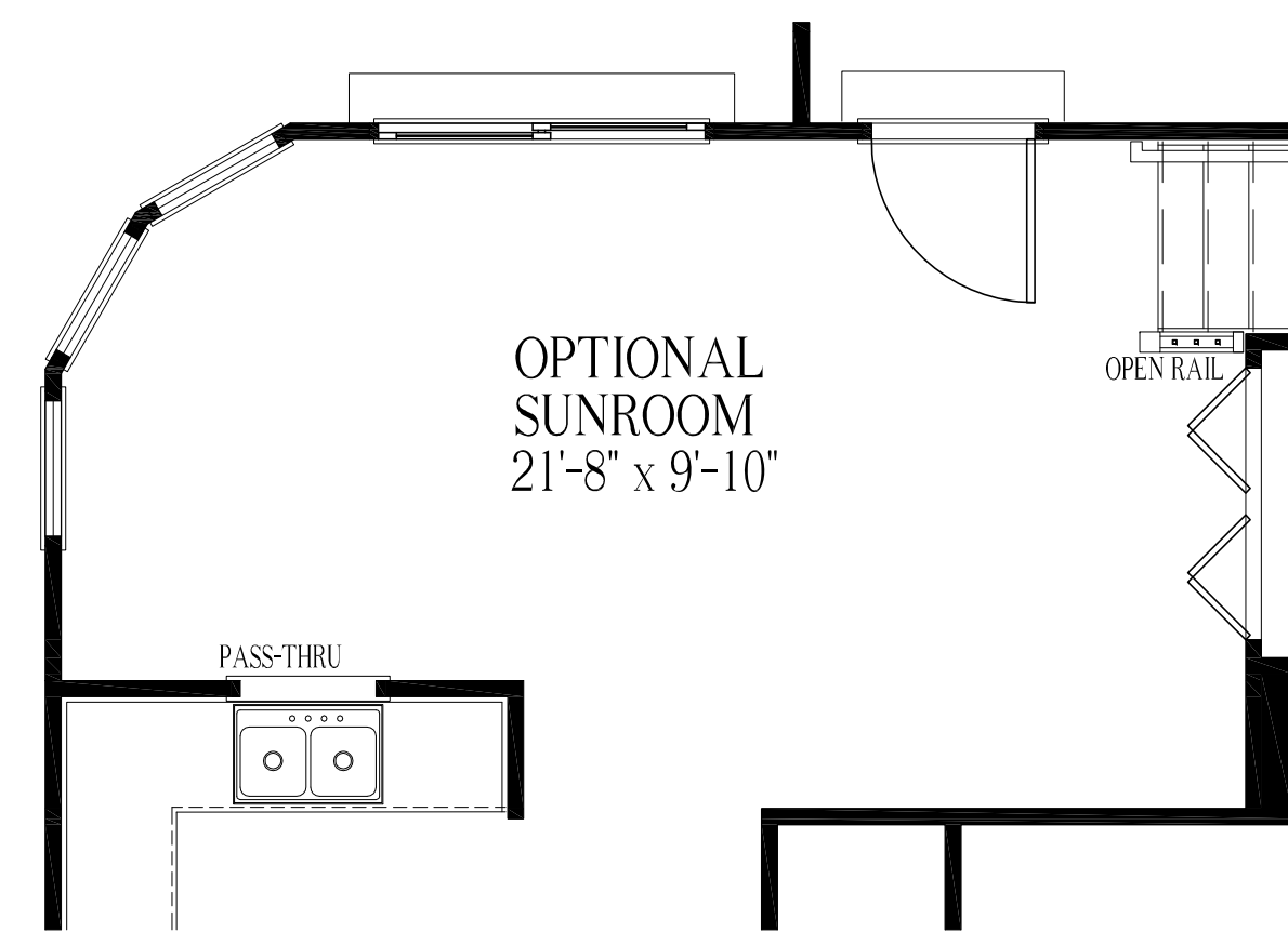
First Floor Plan - Optional Sunroom
