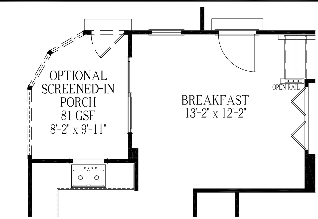
First Floor Plan - Optional Screened-In Porch
