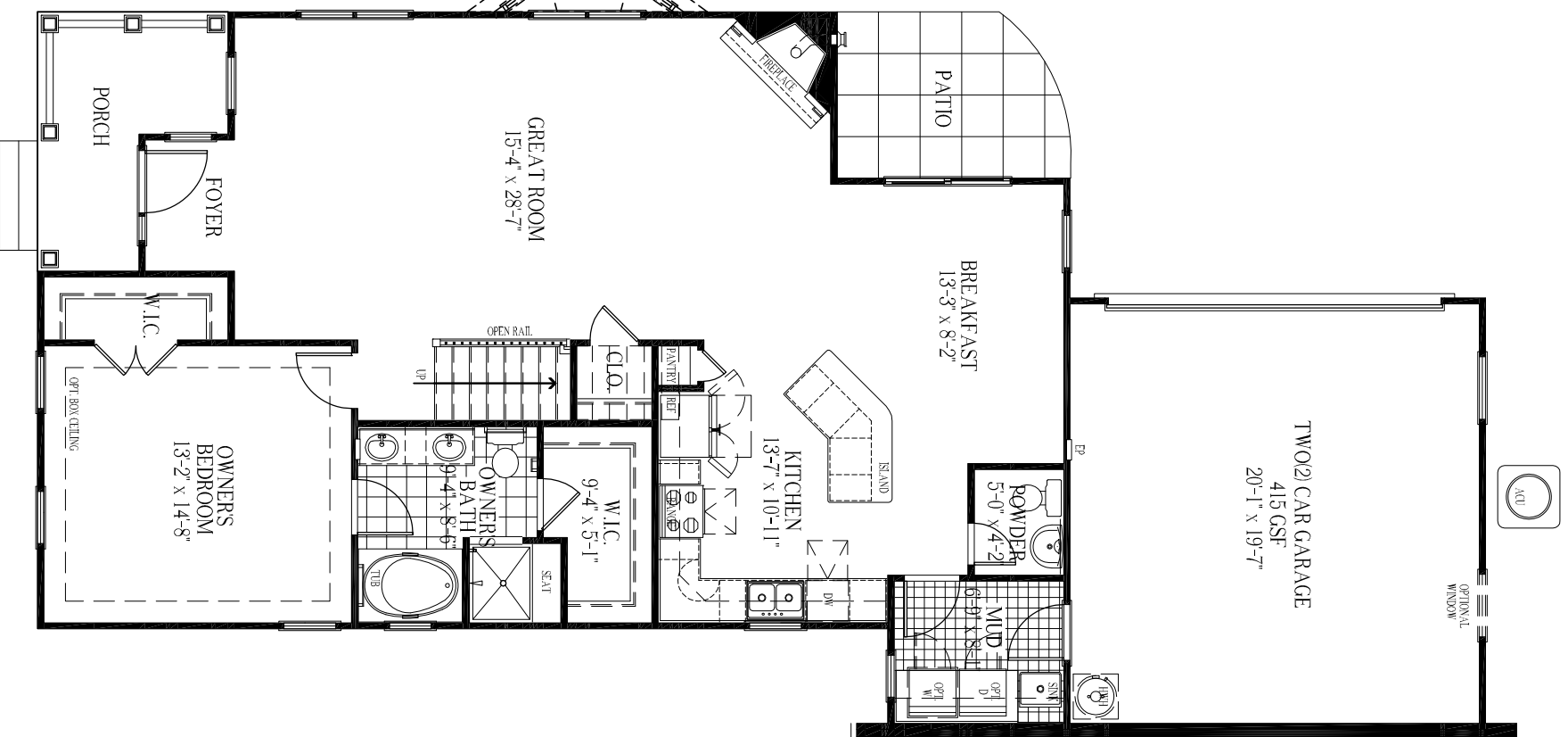
First Floor Plan with Second Floor Elevation 'A' 1,325 GSF
